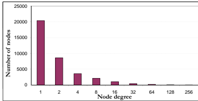
Figure 2: Degree distribution for MOVIES.
